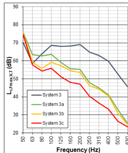
Figure 5. Laboratory impact sound level for the rubber ball, for System 3 with different ceiling configurations.
