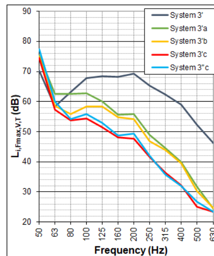
Figure 8. Laboratory impact sound level for the rubber ball, for System 3 with different ceiling and floor covering configurations.
