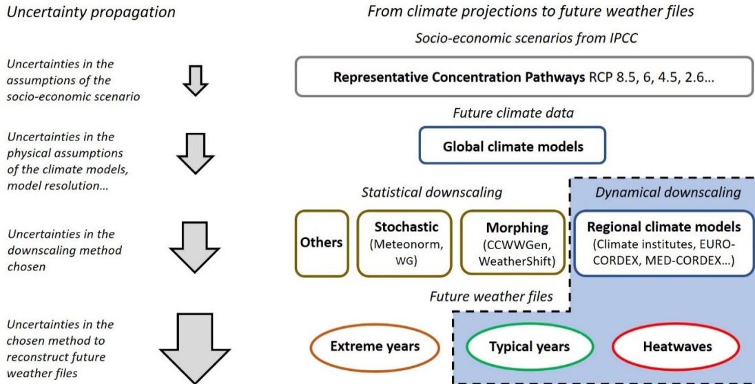
Figure 5. Uncertainty propagation along the modelling chain from multi-years climate projections to future weather files. IPCC: Intergovernmental Panel on Climate Change.
