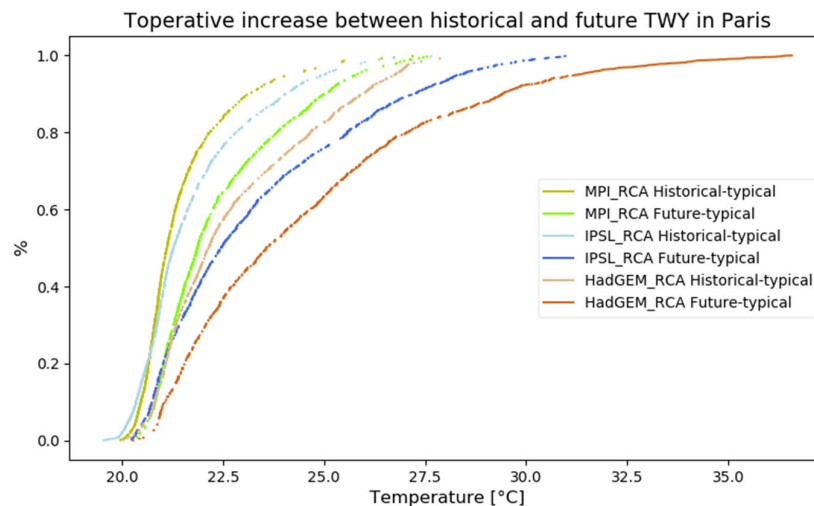
Figure 15. Summer operative temperature increase in the building case study between the historical (1976–2005) and future (2041–2070 RCP 8.5) TWY (typical years) in Paris from the three RCMs.
