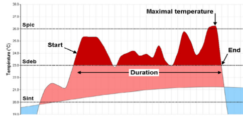
Figure 10. Heatwave detection from [67]. The Spic threshold is used for heatwave detection, the Sdeb threshold defines the heatwave duration, the Sint threshold ends the heatwave. Global intensity: read area of the plot in degree hours.
