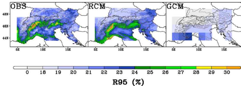
Figure 2. Fraction of total precipitation above the 95th percentile (R95) over the Alpine region. Units are in percent of total precipitation and the simulation period is 1975–2004. OBS = observations, RCM = regional climate model, GCM = global climate model; Adapted from [45].
