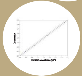
Figure 2: Regression line between the real concentration and the predicted one for NaCl
