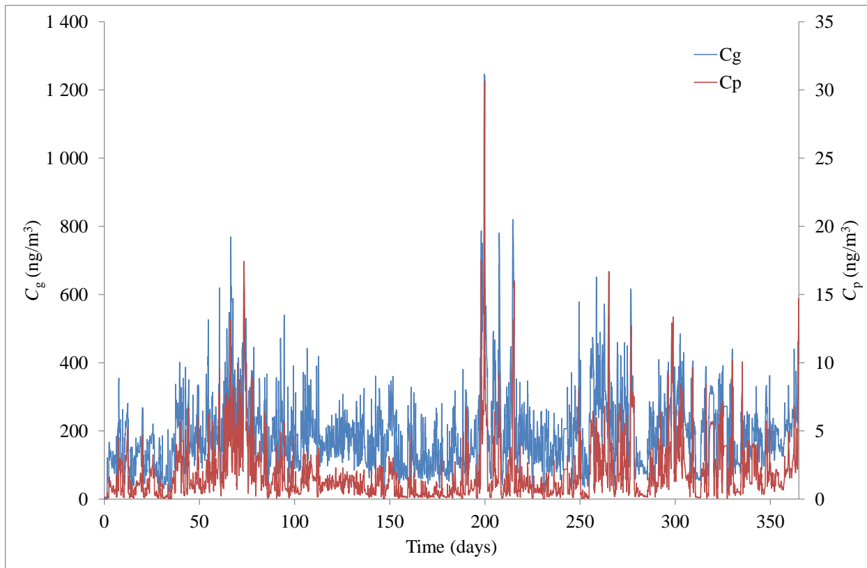
Fig. 5. Predicted hourly average BBzP concentrations in the gas phase ( C_g ) and airborne particles ( C_p ) in a newly built room.
