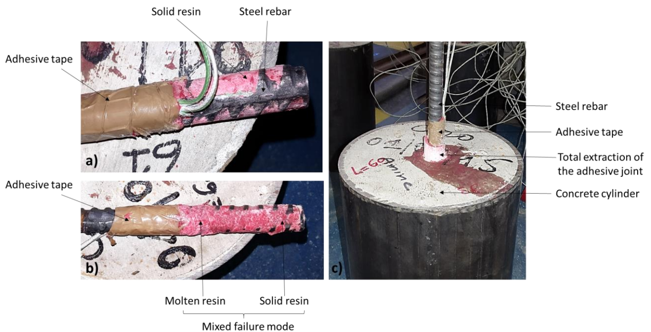
Figure 14: Examples of different failure modes observed during pull-out tests. a) Steel rebar/resin interface (21°C), b) Mixed failure mode (65°C), c) Resin/concrete interface (100°C)
