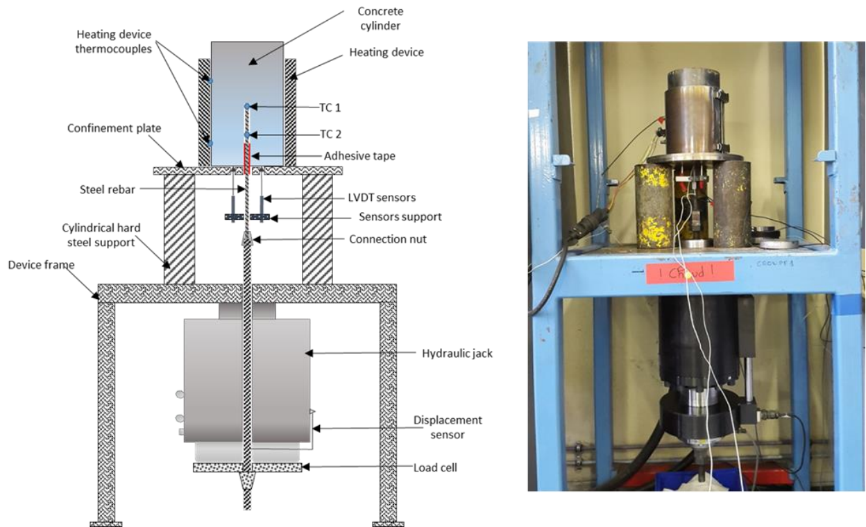
Figure 7: Pull-out experimental device
