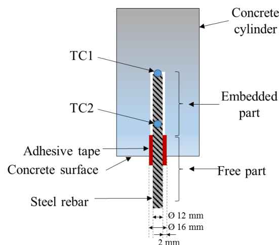
Figure 2: Position of thermocouples and adhesive tape on the anchor
