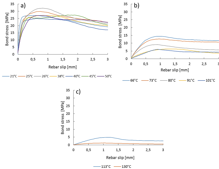
Figure 12: Bond stress vs rebar slip for stabilized temperatures at different ranges a) Target temperatures between 20°C and 50°C, b) Target temperatures between 50°C and 105°C, c) Target temperatures higher than 105°C
