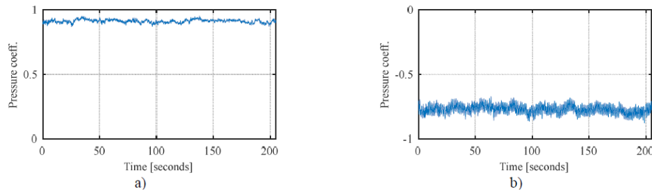
Figure 10 – Time-histories of pressure measured at sensors (a) P10 and (b) P3 during the time interval under analysis.
