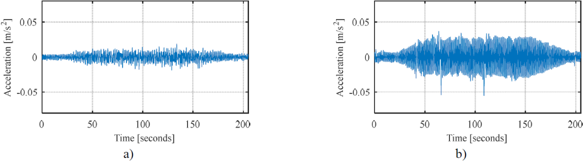
Figure 5 – Time-histories of (a) horizontal and (b) vertical acceleration during the period under analysis.
