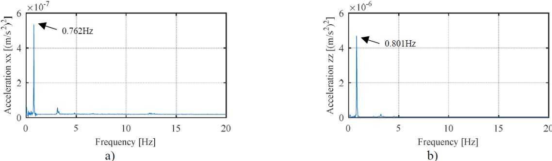
Figure 7 – Spectral estimates of time-histories of (a) horizontal and (b) vertical acceleration.
