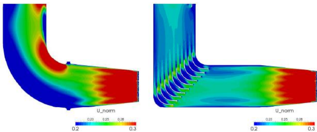
Figure 8: Visualization of the velocity field in the environmental test section – SC1 vs future wind tunnel
