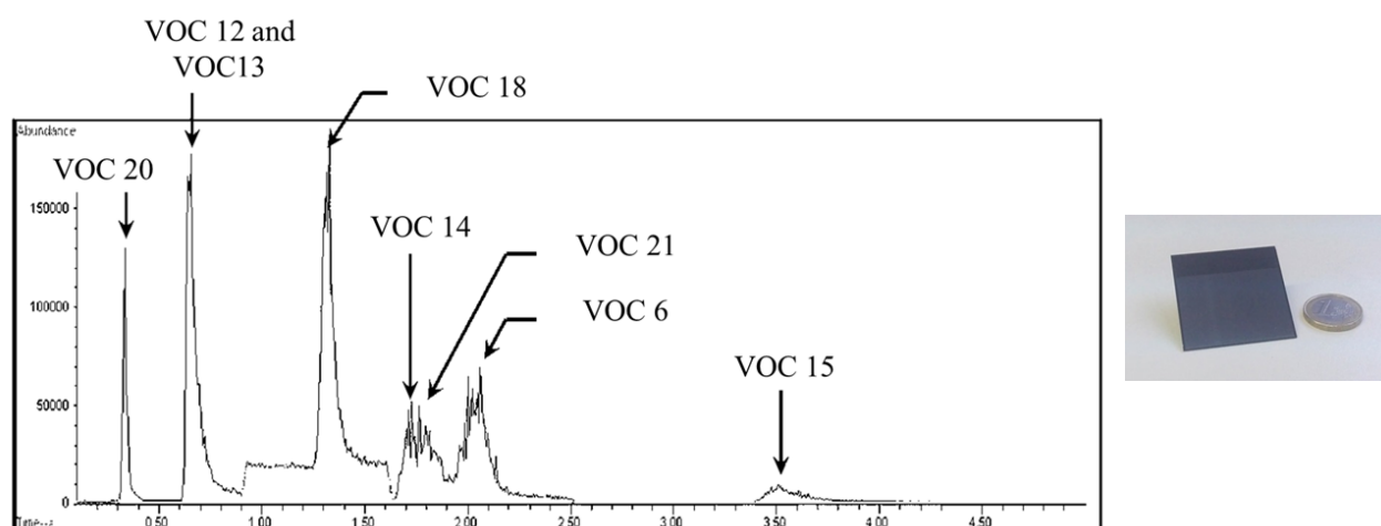
Figure 2: Chromatogram from emissions of a chamber containing 8 fungal VOC's and photograph of separation module
