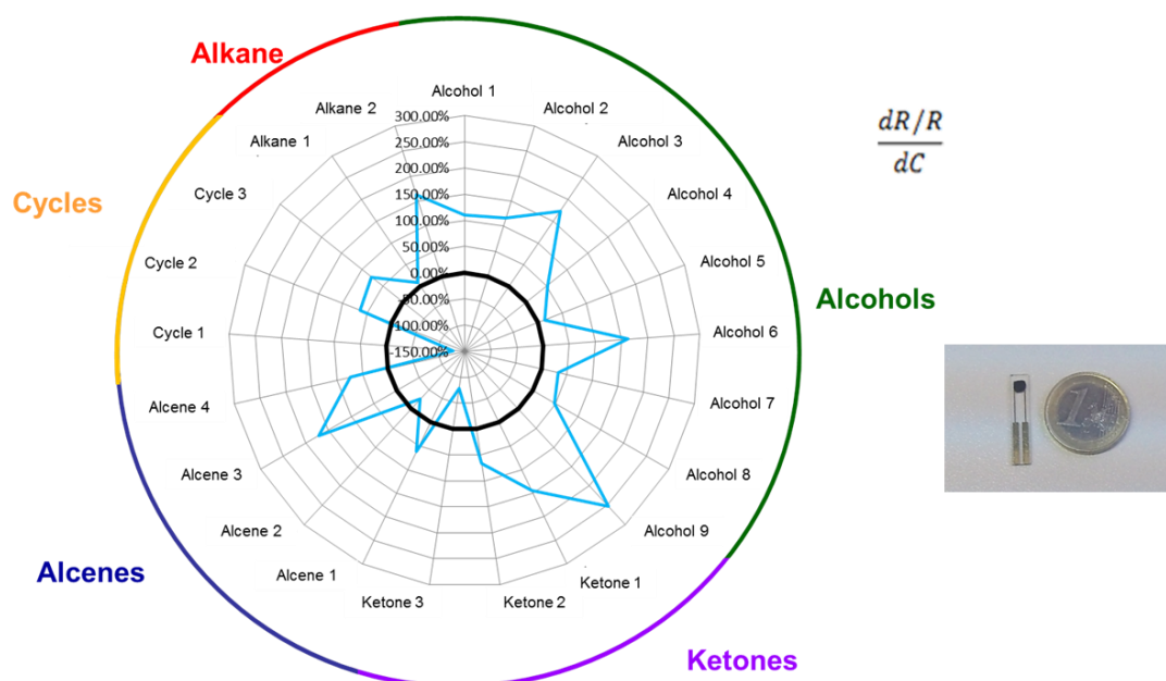
Figure 3: Radar chart for the sensitivity of a polymer for different VOC's and photograph of a polymer sensor
