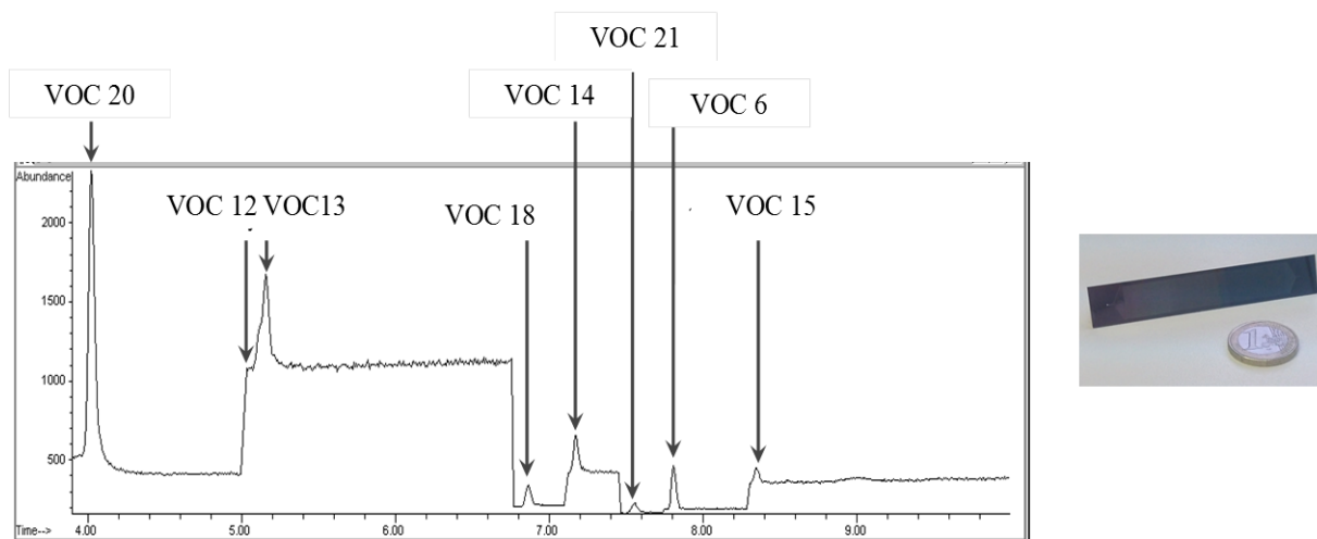
Figure 1: Chromatogram from emissions of a chamber containing 8 fungal VOC's (separation on a standard column) and photograph of the concentration module
