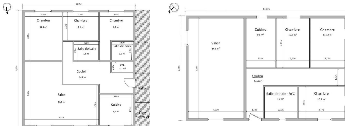
Figure 2. EC-R buildings representation (left: multiple-dwelling, right: individual)
