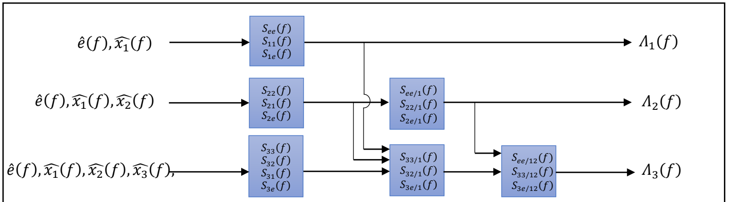
Figure 3: Computation scheme of input's contribution to S_{ee}(f) by PCM method in case of a 3 inputs model.
